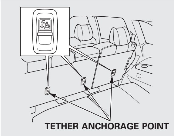
Outer Seating Position
